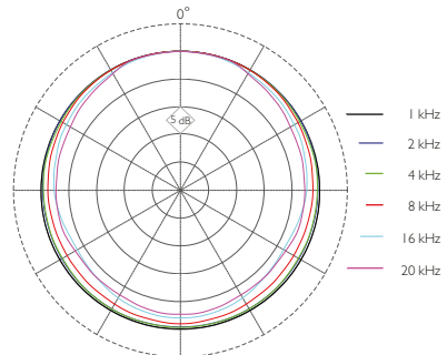
Typical directional characteristics of a 4671 Heavy Duty
